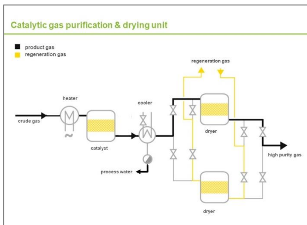
Simplified diagram of Oxygen purification
