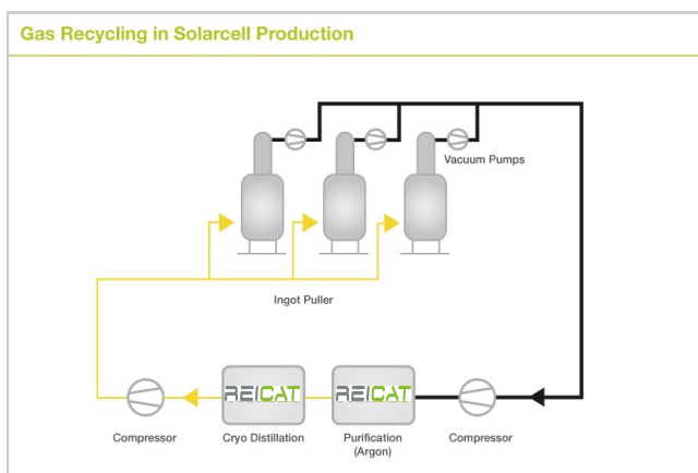
Schematic Mono crystallizer
